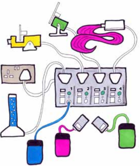
4-channel radio remote unit. All channels can be individually set in any mode and operated separately, manually and radio remotely.
