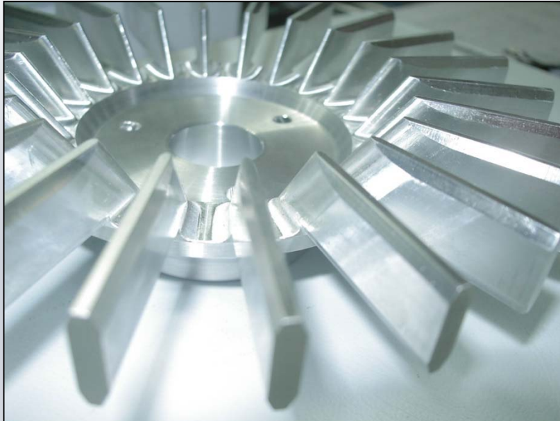
Prototype Pump Impeller to special fluids Material: Aluminium 7075
