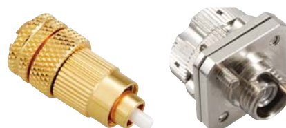
Plug & Bulkhead Variable Attenuator
