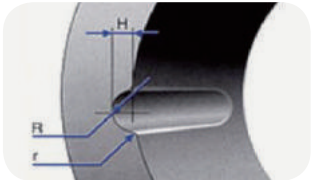
Cross sectional configuraton of oil groove
