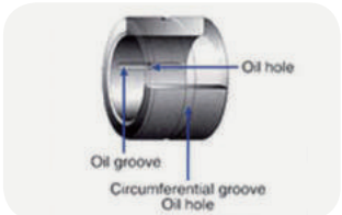
Oil hold and oil groove
