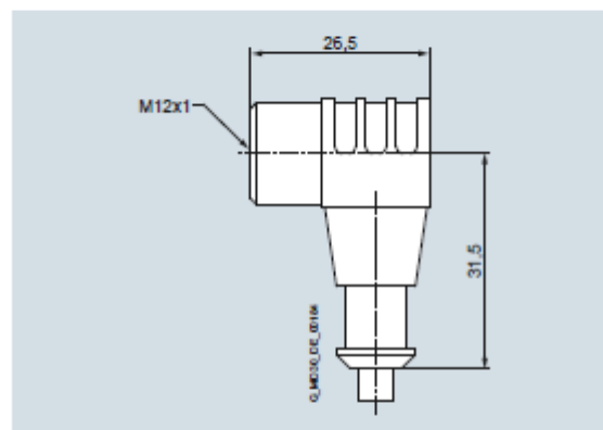
Round connector WWAK4.21-2/P00
