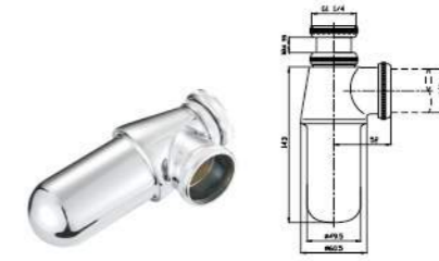
Code: Y00167 Spec: 1.1/4" x 40mm Bottle Trap Siphon
