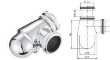
Code: Y00166 Spec: 1.1/4" x 32mm Bottle Trap Siphon
