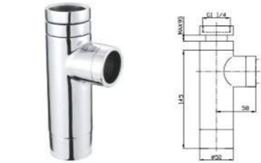
Code: Y00165 Spec: 1.1/4" x 35mm Bottle Trap Siphon
