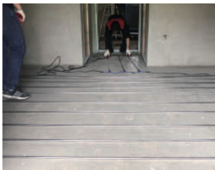
02 Ondol arrangement
