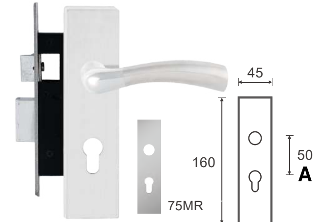
Semi Mortise 75MH-250 SS
