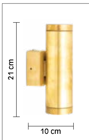
SPOT LIGHT 60.2/F BRASS
