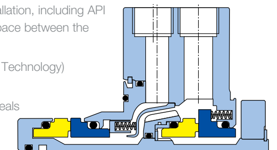
AESSEAL® CAPI-TXS™ Type A Dual Seal
