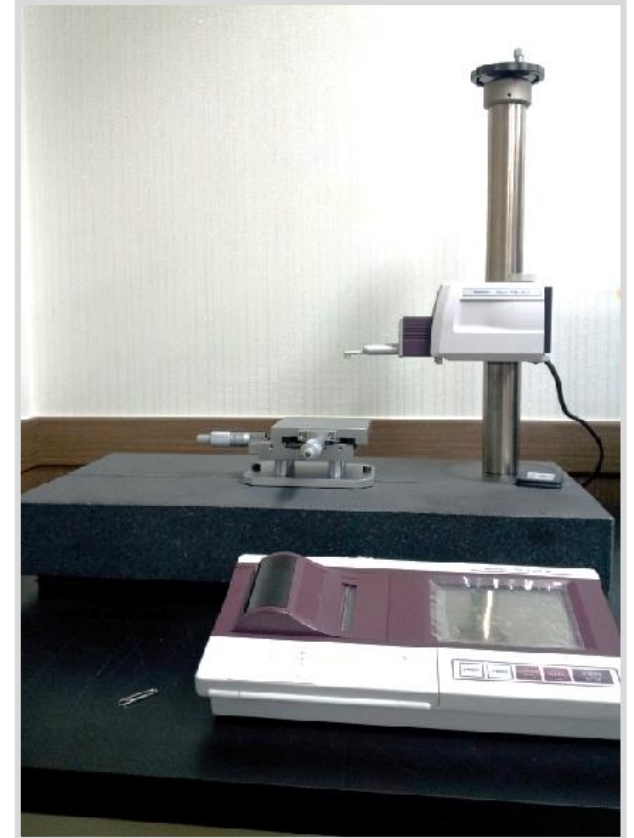
Roughness tester
