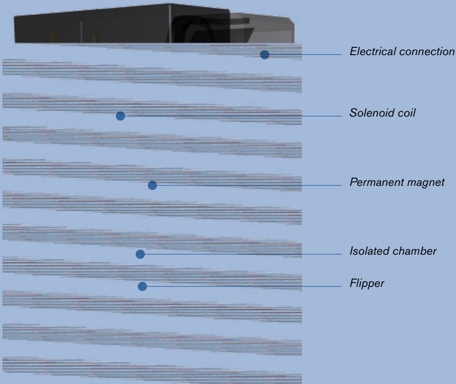
Direct acting 3/2-way flipper valve type 6144
