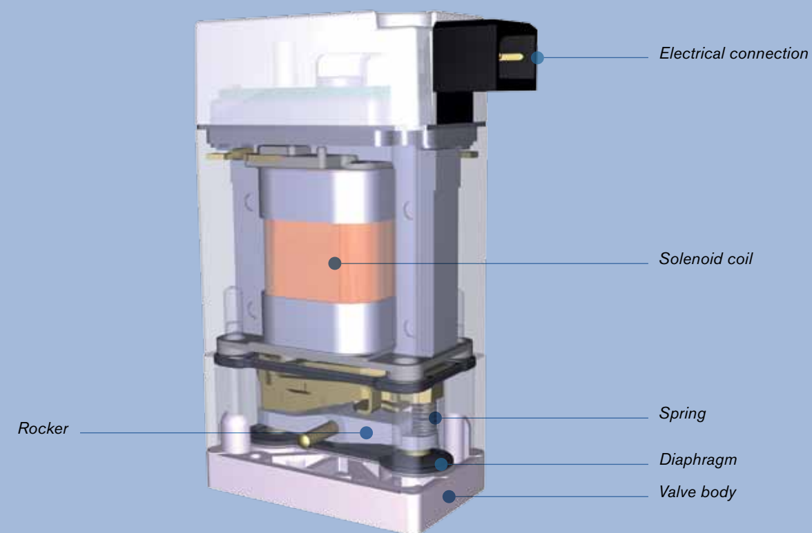
Direct acting 3/2-way rocker valve type 0127
