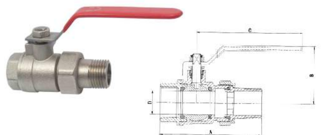
Lever ball valve FxM
