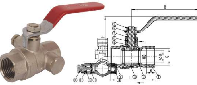
Lever ball valve
