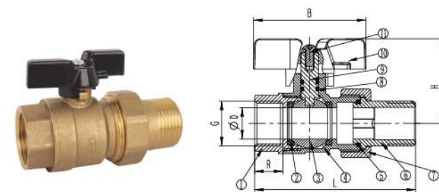
Tee handle ball valve FxM brass
