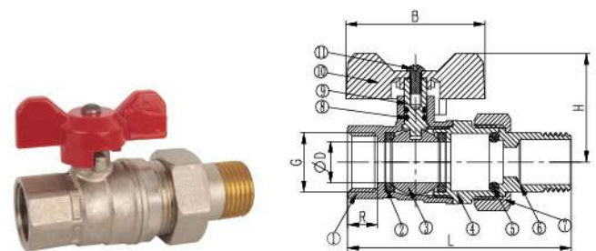
Tee handle ball valve FxM
