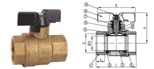
Tee handle ball valve FxF brass
