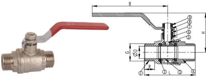
Lever ball valve MxM
