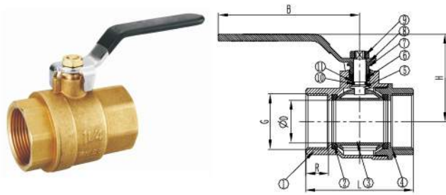
Lever ball valve FxF brass
