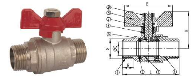
Tee handle ball valve MxM
