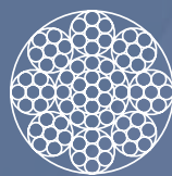
8 x 19+7 x 7
