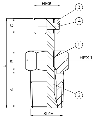
Components List
