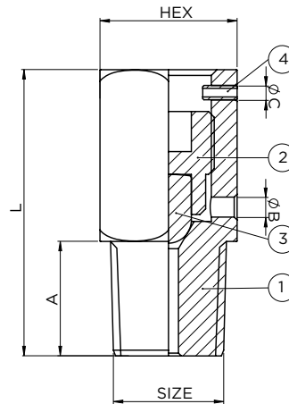
Components List
