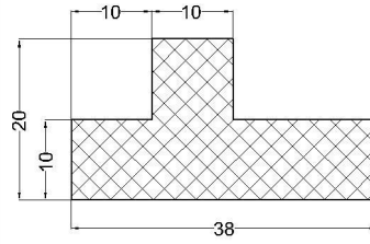
cod:VLC 07-050 material: cauciuc siliconic 60°Sh
