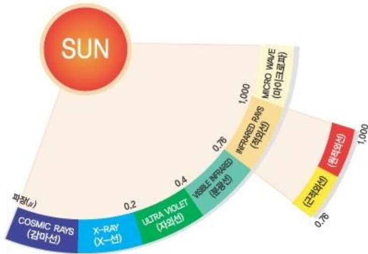
태양광선 분광표 (Electromagnetic Spectrum of Sunlight)
