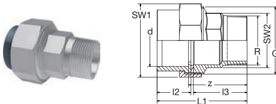
621.54.07 PVC-U-V2A Ü-Verschraubung AG-keg Flachdichtring-EPDM grau PVC-U-Stainless Steel Transition-Union male-thread-con flat-gasket-EPDM grey
