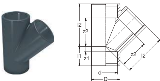
621.25.01 PVC-U Abzweig 45° grau PVC-U Branch 45° grey
