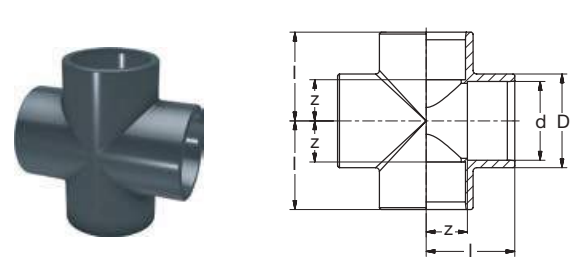
621.30.01 PVC-U Kreuz grau PVC-U Cross grey
