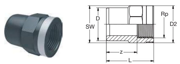
621.91.04 PVC-U Ü-Reduktion IG-zyl grau PVC-U Transition-Reducer female-thread-cyl grey
