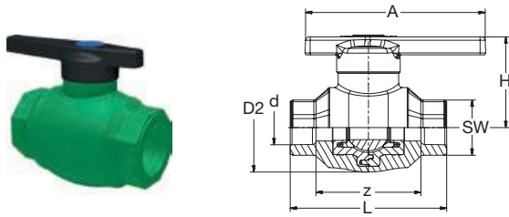
G 8850B PP-RCT Kugelhahn 20°C/1.0MPa grün PP-RCT Ball valve 20°C/1.0MPa green
