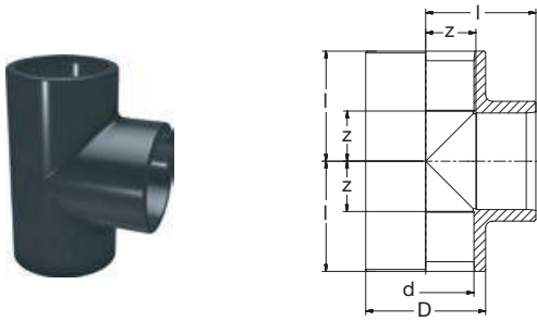
621.20.01 PVC-U T-Stück 90° grau PVC-U Tee 90° grey
