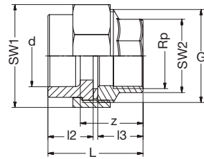
G 8542g PP-R-V2A Ü-Verschraubung IG-zyl Flachdichtring-EPDM 20°C/1.0MPa grün PP-R-Stainless steel Transition-Union female-thread-cyl flat-gasket-EPDM 20°C/1.0MPa green
