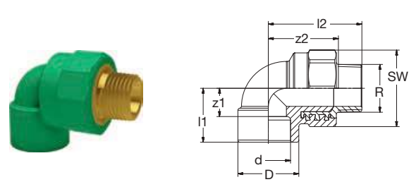
G 8092gB PP-RCT-RG Ü-Winkel 90° AG-keg grün PP-RCT-Bronze Transition-Elbow 90° male-thread-con green
