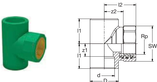
G 8130gB PP-RCT-RG Ü-T-Stück 90° IG-zyl grün PP-RCT-Bronze Transition-Tee 90° female-thread-cyl green
