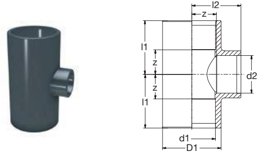
621.20.01 PVC-U T-Stück 90° red grau PVC-U Tee 90° red grey
