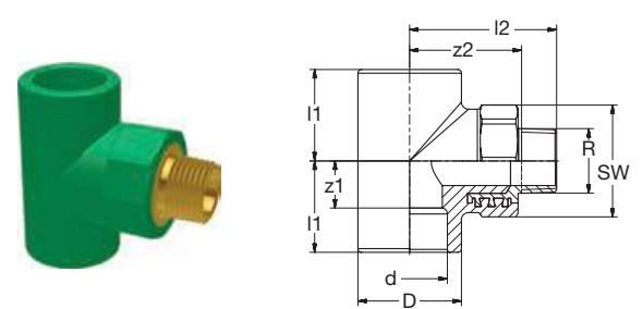
G 8133gB PP-RCT-RG Ü-T-Stück 90° AG-keg grün PP-RCT-Bronze Transition-Tee 90° male-thread-con green
