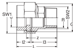
G 8547g PP-R-V2A Ü-Verschraubung AG-keg Flachdichtring-EPDM 20°C/1.0MPa grün PP-R-Stainless steel Transition-Union male-thread-con flat-gasket-EPDM 20°C/1.0MPa green
