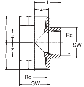
621.20.16 PVC-U T-Stück 90° IG-keg grau PVC-U Tee 90° female-thread-con grey
