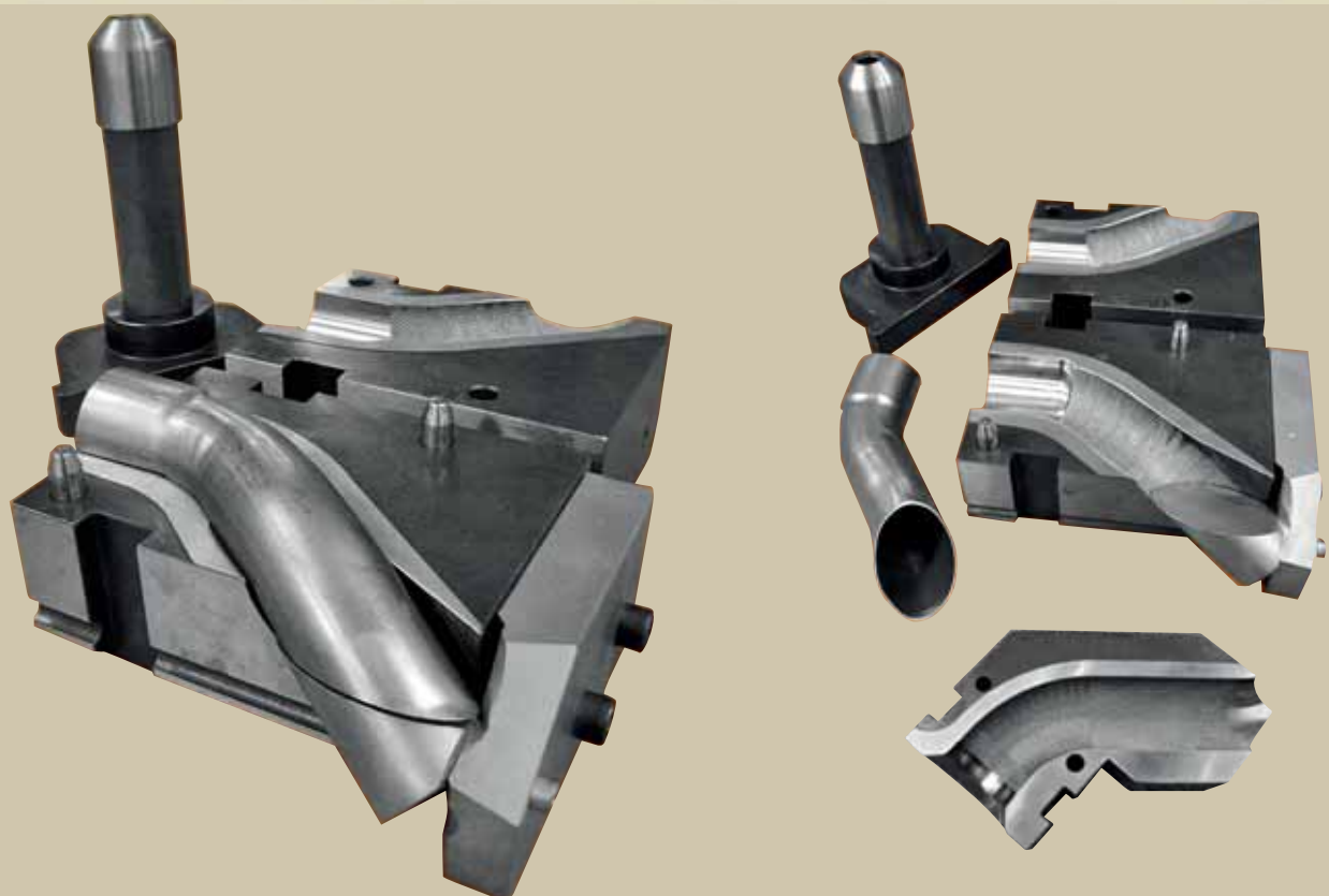
Wedges for flaring pipe ends .
