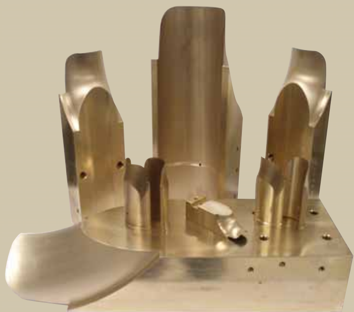
Different counter rail models For pipes of up to \varnothing 18 200
