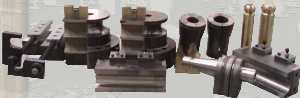
2-height dies, clamps, mandrels and rails.
