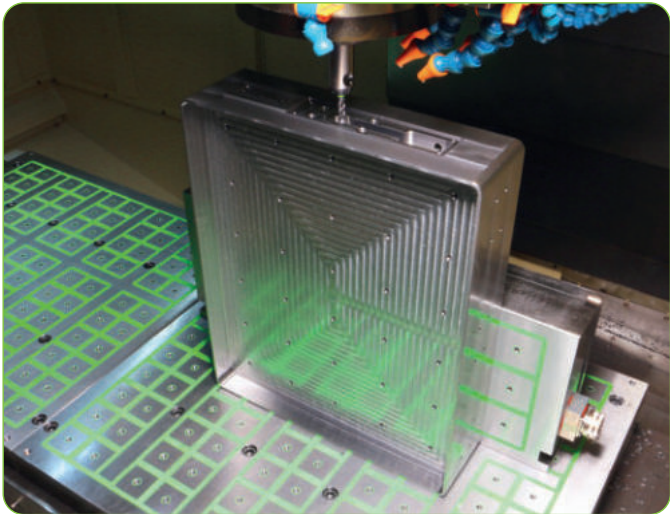
Vertical clamping surface on 3-axis machines
