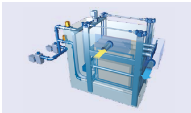
The cloth media filter is a compact high-capacity process for tertiary filtration (down to 5 to 10 microns) that enables reuse of treated wastewater for many purposes.
