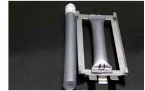
Zero hour sample (prior to exposure) and a sample subjected to an accelerated ageing test after 4000 hours of exposure.
