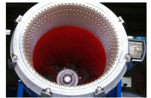
Nozzle System
