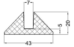
cod:VLC 07-124 material: SBR 70°Sh
