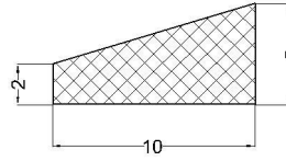
cod:VLC 07-195 material: cauciuc siliconic 70°Sh
