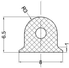
cod:VLC 07-193 material: cauciuc siliconic 50°Sh
