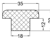
cod:VLC 07-206 material: cauciuc siliconic 65°Sh alimentar
