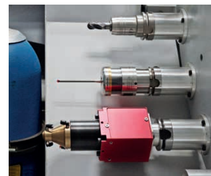
Tool, measuring probe and fibre laser unit in the tool changer
